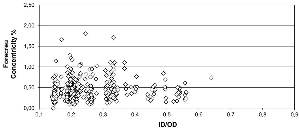
Forecreu concentricity % versus ID/OD
