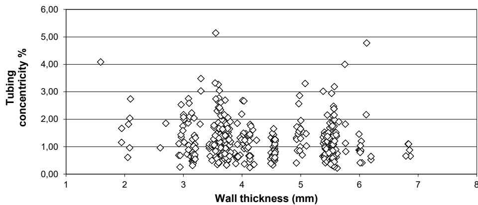
Tubing concentricity % versus wall thickness
