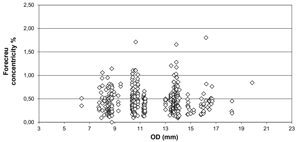
Forecreu concentricity % versus OD
