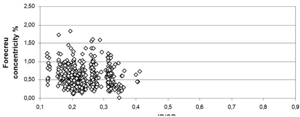
Tubing concentricity % versus wall thickness
