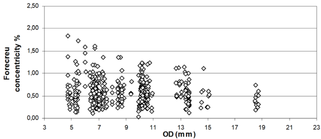
Forecreu concentricity % versus OD
