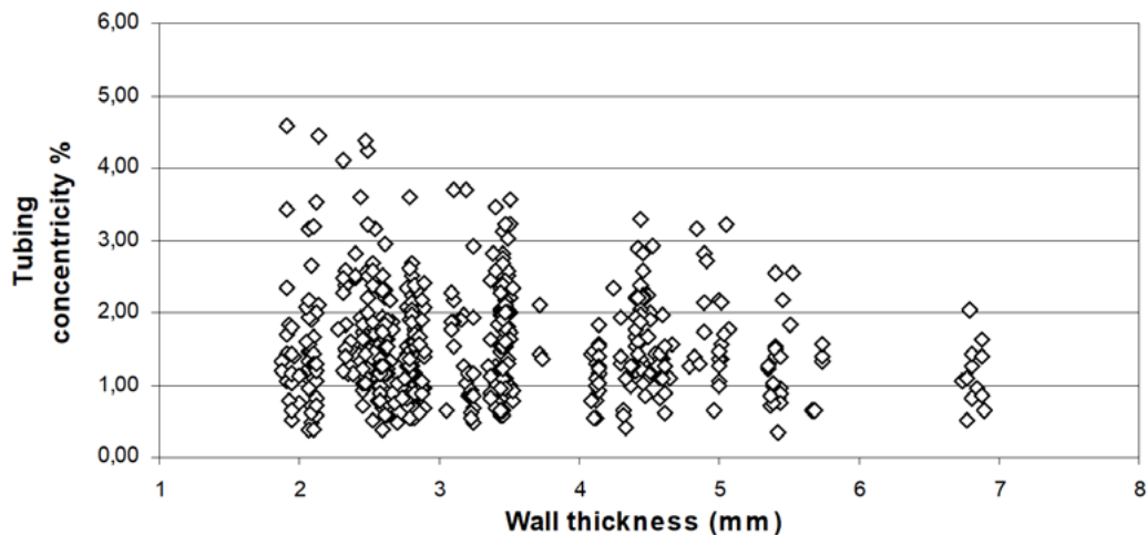
Tubing concentricity % versus wall thickness
